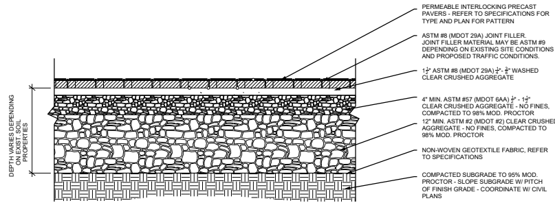
POROUS PAVERS DETAIL NOT TO SCALE
