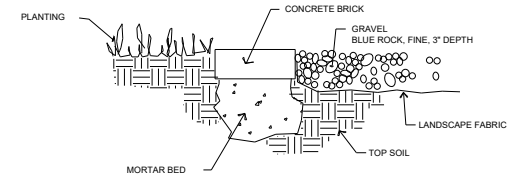
BRICK HEADER DETAIL NOT TO SCALE
