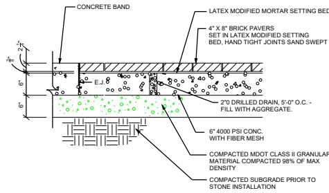
BRICK PAVER ON CONCRETE BASE DETAIL NOT TO SCALE
