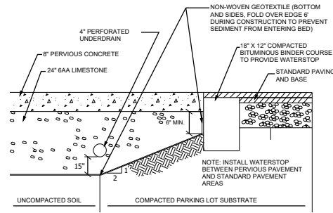
POROUS CONCRETE DETAIL NOT TO SCALE
